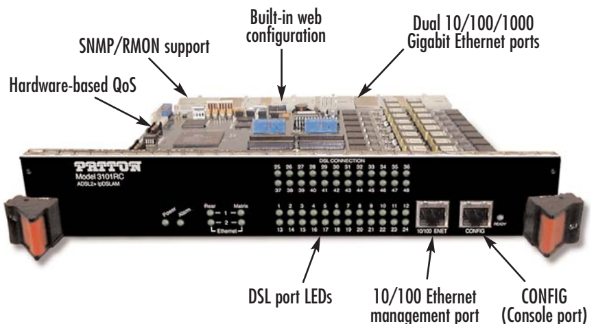
3101RC Triple Play IPDSLAM
