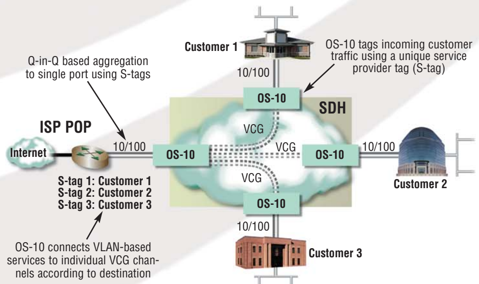
Figure 12. LAN extension service using VLAN trunking
