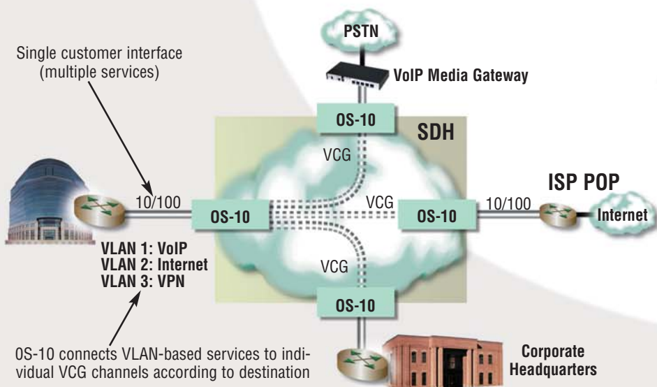
Figure 11. LAN extension service by mapping VLANs to VCAT groups
