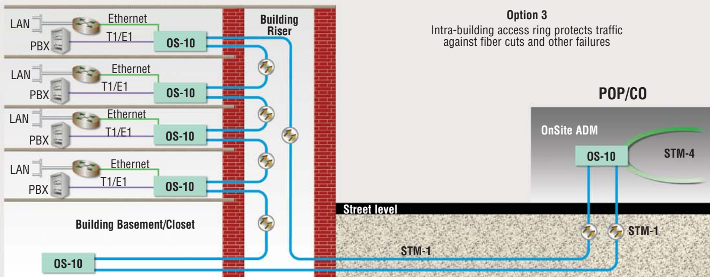
Figure 14. Deployment option 3: Intra-building ring using the OS-10
