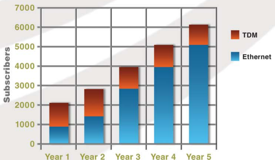
Figure 1. Services evolution
