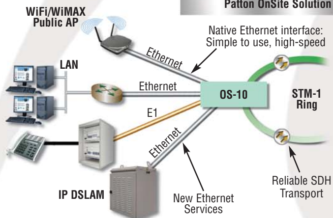
Figure 10. Migration from PDH to Ethernet leased-line services using the OnSite
