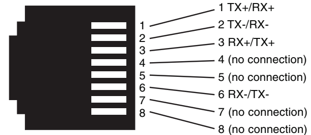
Figure 5. Model 1069 10/100Base-T RJ-45 Connector Pinout.
