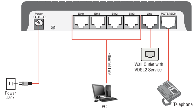
Figure 3. Model 1069 connection diagram
