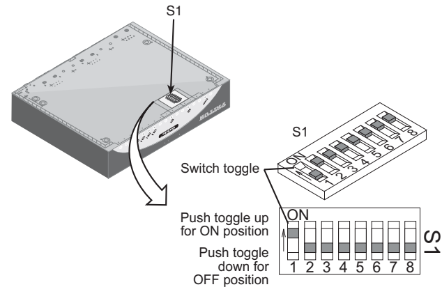
Figure 7. DIP switch orientation
