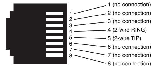
Figure 6. Model 1069 (RJ-45) POTS/ISDN interface.
