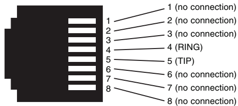
Figure 4. Model 1069 (RJ-45) twisted pair line interface.
