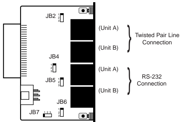
Figure 4. Strap locations for both rear cards
