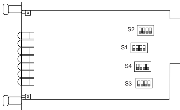
Figure 1. Model 1004ARC Card, showing location of configuration switches.
