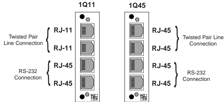
Figure 3. Model 1004ARC interface card options
