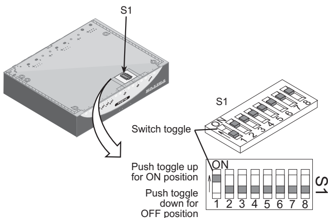
Figure 7. DIP switch orientation
