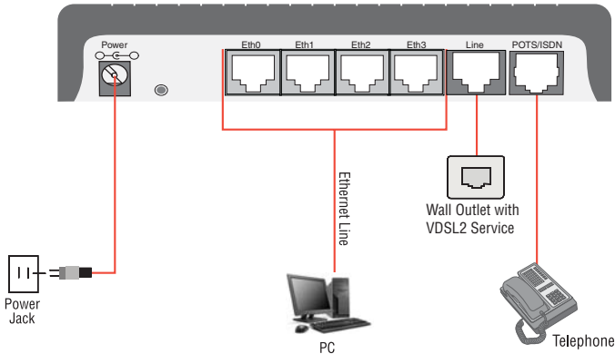
Figure 3. Model 1069 connection diagram
