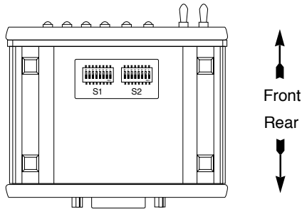
Figure 1. Underside of the 1075 Showing Location of DIP Switches
