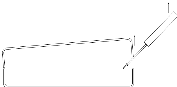
Figure 4. Opening the 1075 Case With a Small Screwdriver
