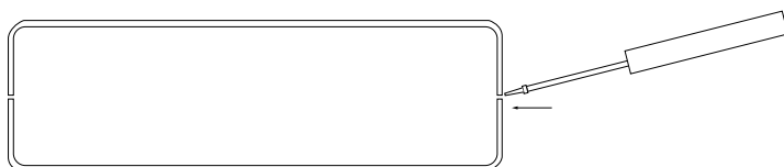
Figure 3. Opening the 1075 Case with a Small Screwdriver
