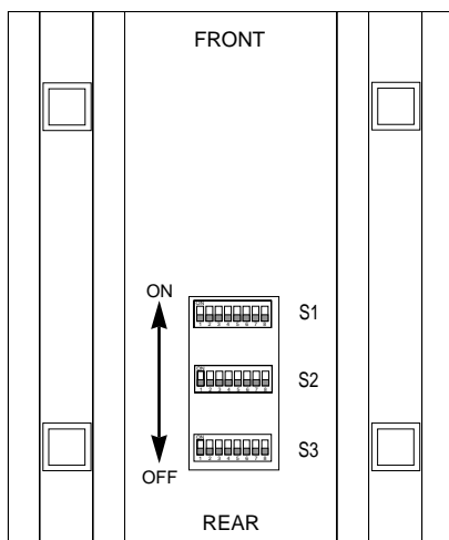
Figure 1. Underside of Model 1080A Series, showing location of DIP switches
