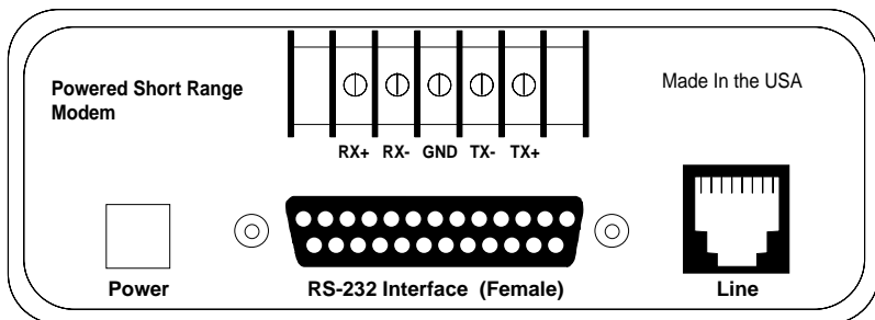
Figure 3. Rear view of Model 1080A Series
