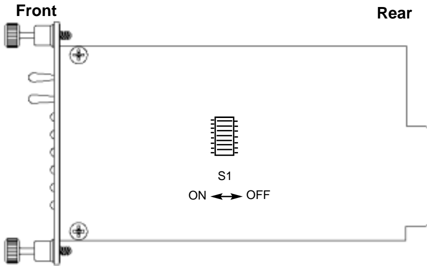
Figure 2. Underside of Model 1193RC, showing location of the DIP switches
