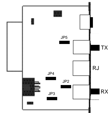
Figure 5: Top view of 1193RC circuit board and location of jumpers
