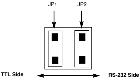
Figure 4: Non-Inverted Data and Control Signal Jumpers
