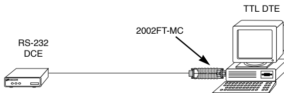
Figure 9. Connecting the Model 2002FT-MC
