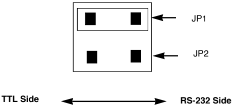
Figure 6: Inverted Data and Non-Inverted Control Signal Jumpers
