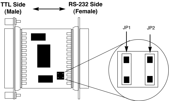
Figure 3: Close-Up of the Model 2002 Series Jumper Straps
