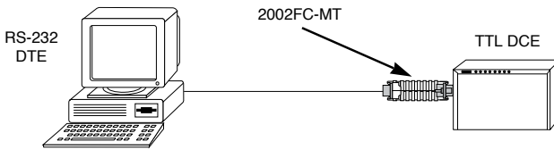
Figure 8: Connecting the Model 2002FC-MT
