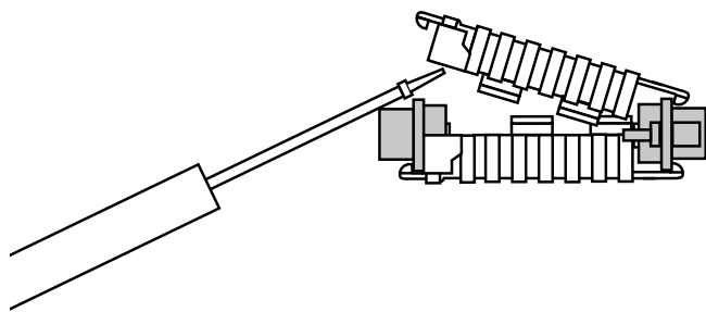
Figure 2: Using a Small Screw Driver to Open the Model 2002 Case
