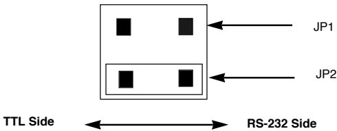
Figure 7: Inverted Control and Non-Inverted Data Signal Jumpers
