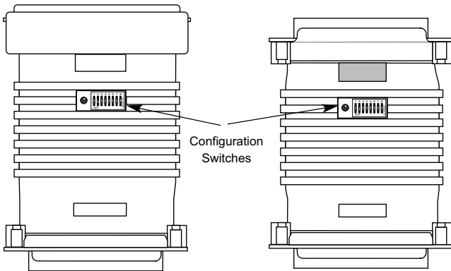
Figure 1. The location of the configuration switches: the Model 2036 (left) and the Model 2037 (right)
