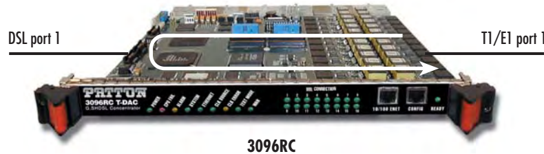
Figure 46. Local loopback
