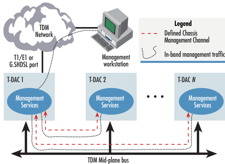
Figure 82. In-band management
