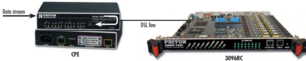
Figure 58. CPE local loopback
