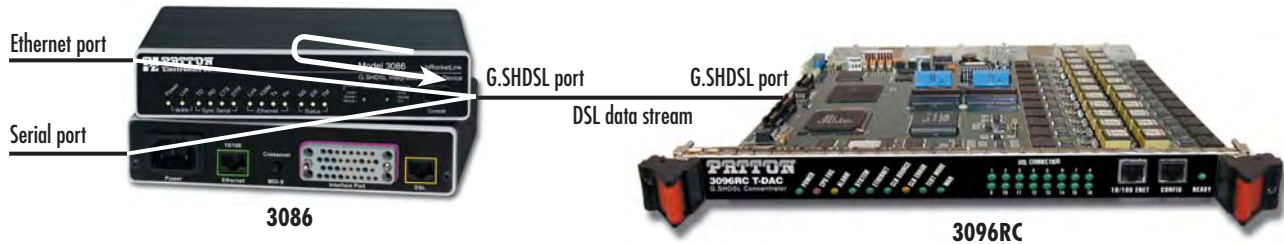
Figure 48. Remote Ethernet loopback
