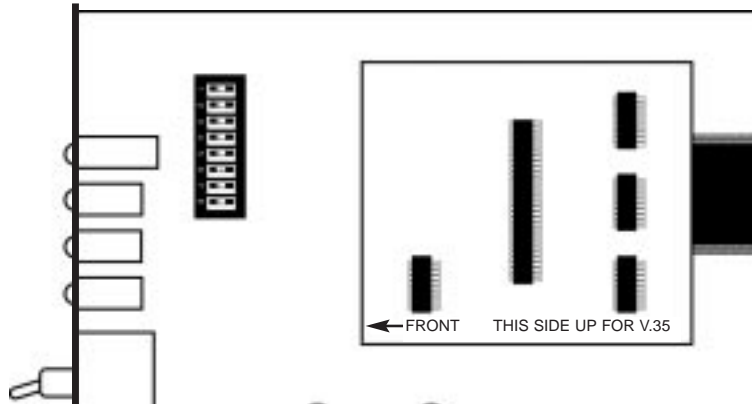
Figure 3. Closeup of Model 2703RC-A Interface Driver Board
