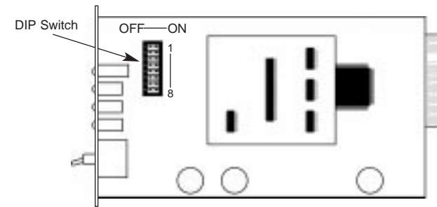
Figure 1. Model 2703RC-A board, showing switch locations
