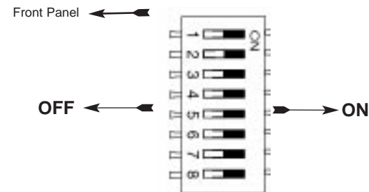
Figure 2. Close up of the configuration switches NOTE: The OFF position is oriented toward the front of the Model 2703RC-A
