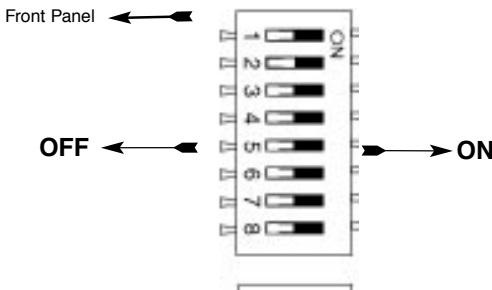
Figure 2. Close up of the configuration switches
