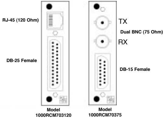
Figure 7. Rear interface card options for the Model 2703RC
