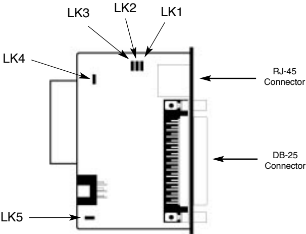
Figure 4. Jumper Locations for the Model 1000RCM703120 Rear Card
