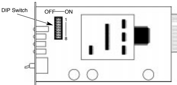
Figure 1. Model 2703RC board, showing jumper locations
