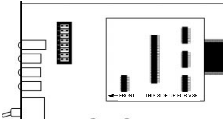
Figure 3. Closeup of Model 2703RC Interface Drive Board
