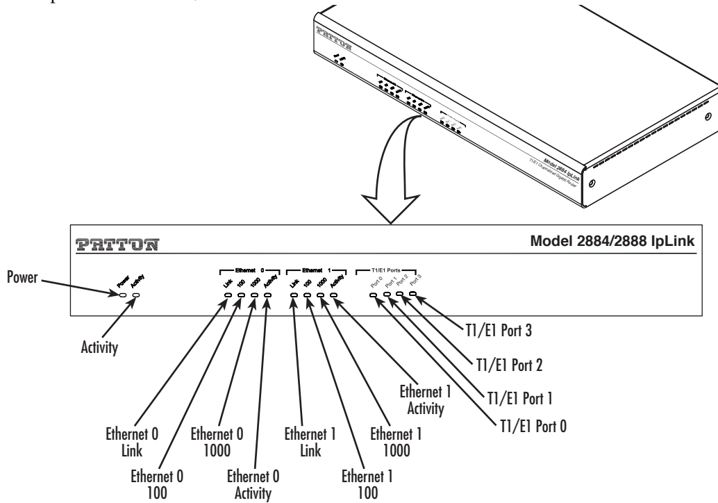
Figure 3. IpLink 2884 front panel
