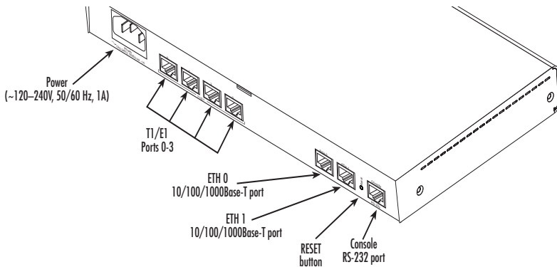
Figure 2. 2884 rear panel
