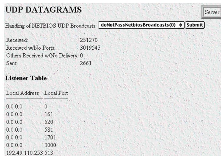
Figure 79. UDP window
