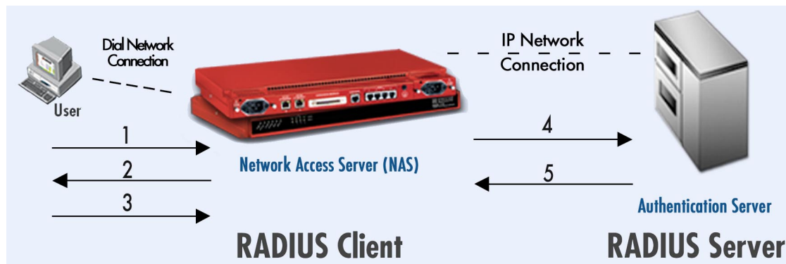
Figure 124. RADIUS authentication and authorization procedure
