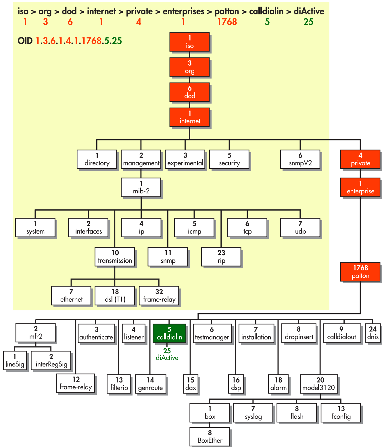
Figure 127. MIB tree for Model 2960 access server
