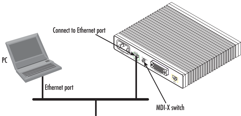
Figure 2. Connecting the ipRocketLink to the local IP network
