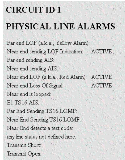
Figure 105. Line Status Alarms window
