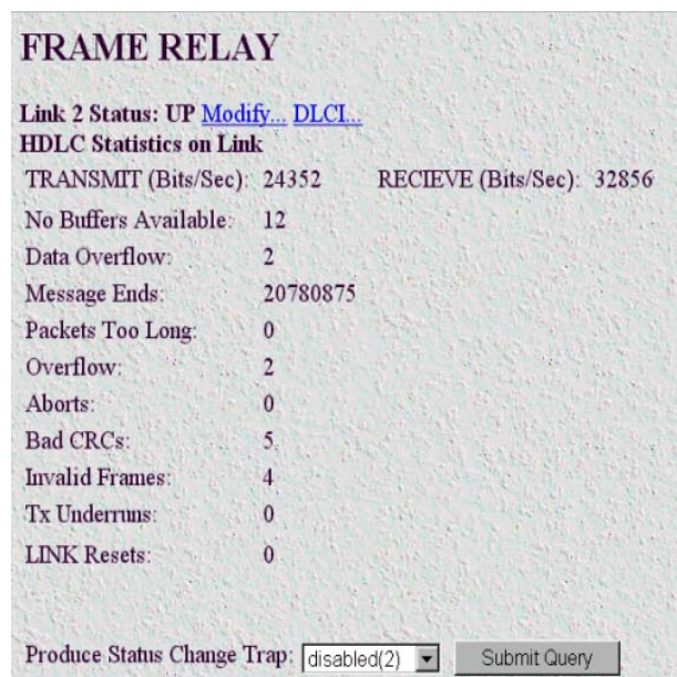
Figure 72. Frame Relay main window
