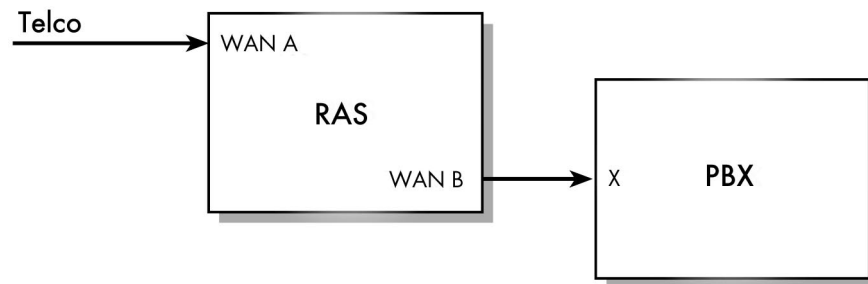
Figure 59. Drop and insert diagram
