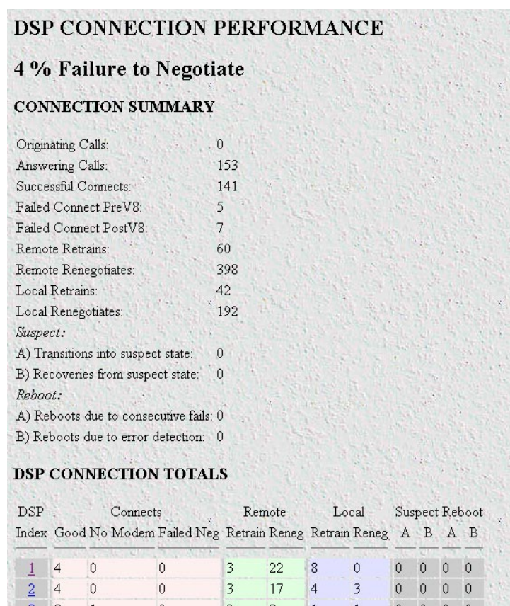
Figure 62. DSP Connection Performance window
