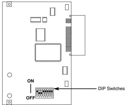
Figure 1. Model IM2RC/F-128K Card Showing DIP Switches
