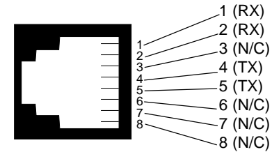
Figure 6: 120 Ohm RJ-45 G.703 Interface
