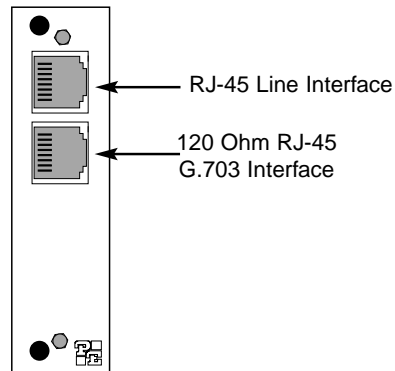
Figure 5: Model IM2RC/F128-K Interface Ports
