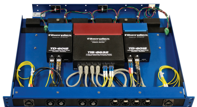
Preconfigured 4 HD-SDI Video plus 10/100/1000 Ethernet
