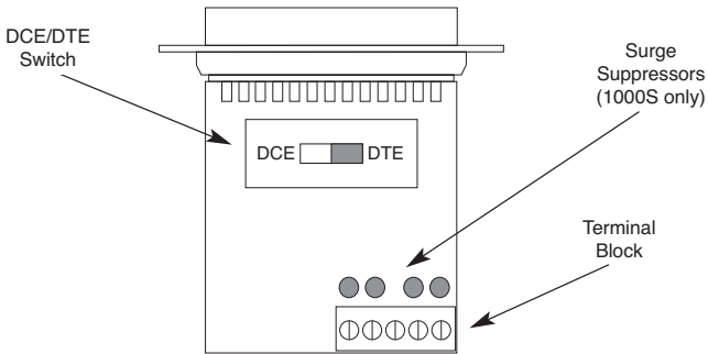
Figure 1: Location of Key Components on Model 1000 Printed Circuit Board
