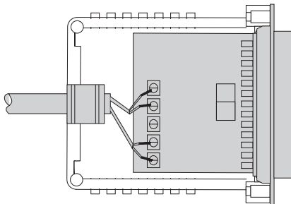
Figure 10: Positioning the Model 1000 Inside the Plastic Case
