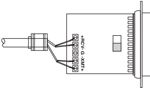
Figure 9: Re-connecting the Strain Relief Assembly
