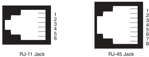
Figure 3. Pin Number Assignments for RJ11 and RJ45 Modular Jacks
