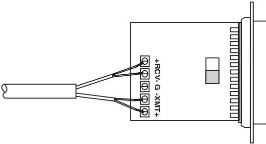
Figure 8: Proper Twisted Pair Connections to the Model 1009 Terminal Blocks
