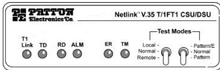
Figure 3: 2720/C Front Panel
