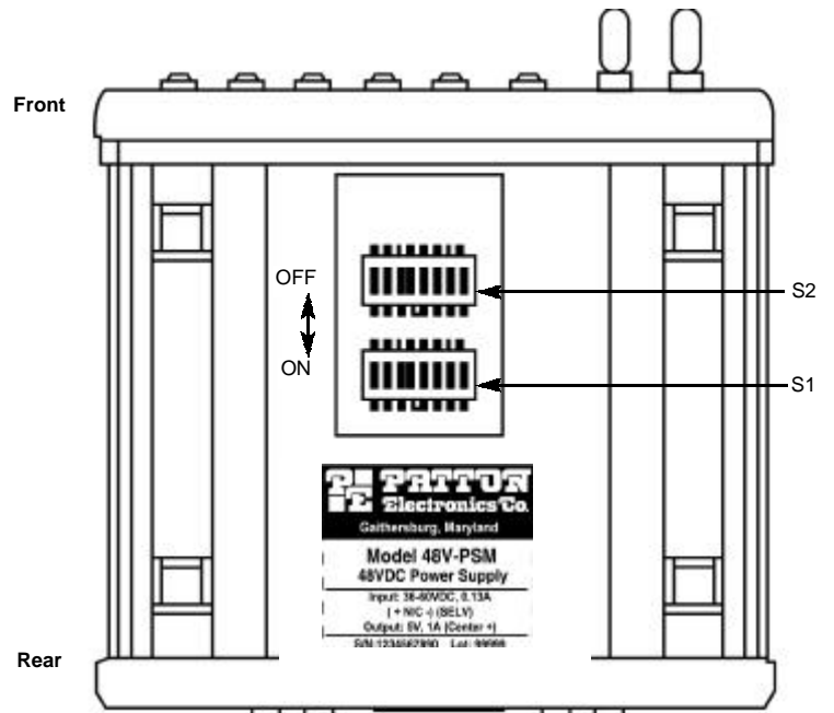
Figure 1. Underside of Model 2720, Showing Location of DIP Switches
