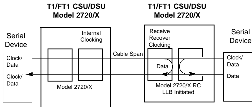
Figure 7. Local Loopback
