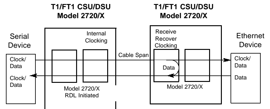
Figure 8. Remote Loopback
