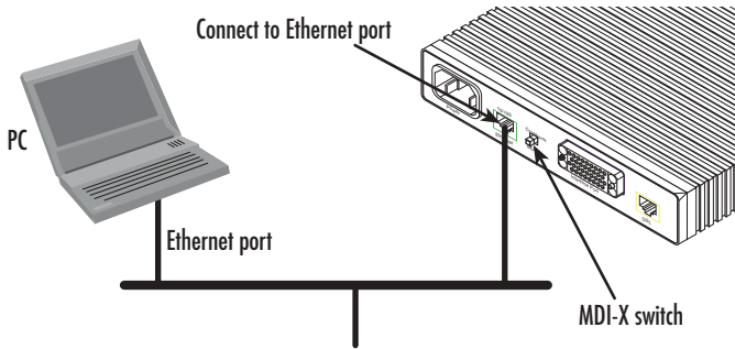
Figure 2. Connecting the ipRocketLink to the local IP network (Model 3086/RIC shown)
